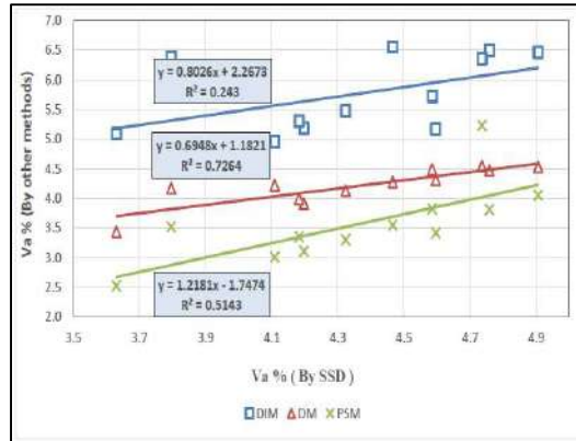
Figure (11): Linear relationship between the air void content obtained by SSD method and other three methods in Dense Asphalt.
